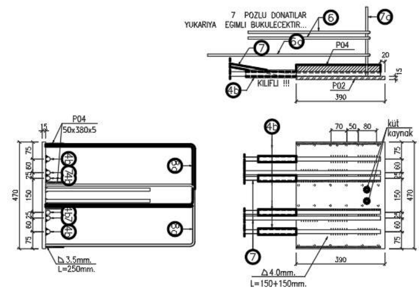
P03 PLAKA DETAYI \nabla 390x470x15 P05 PLAKA DETAYI \nabla 50x370x5
