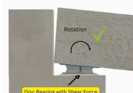
Disc Bearing with Shear Force Resisting Pin (Bridges)
