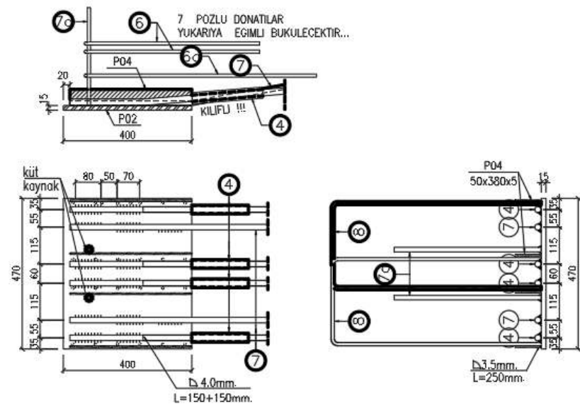
P02 PLAKA DETAYI \nabla 400x470x15 P04 PLAKA DETAYI \nabla 50x380x5
